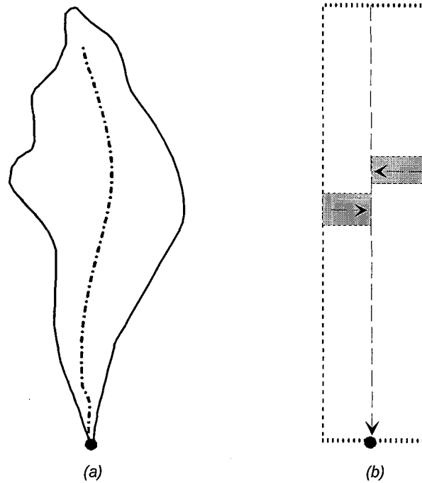
Figure 6-3. Simple watershed with kinematic-wave model representation
