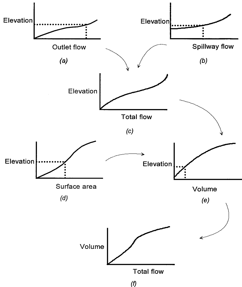
Figure 10-5. Illustration of procedure for defining storage-outflow relationship
