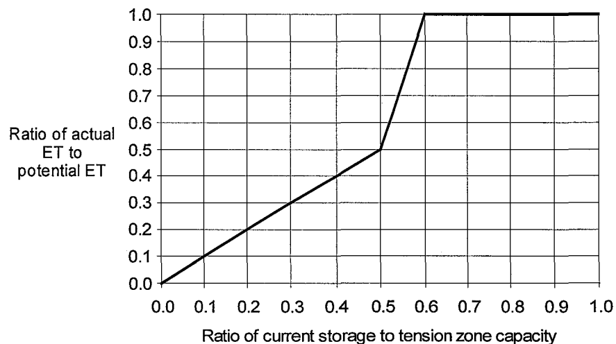
Figure 5-2. ET as a function of tension zone storage (Bennett, 1998)
