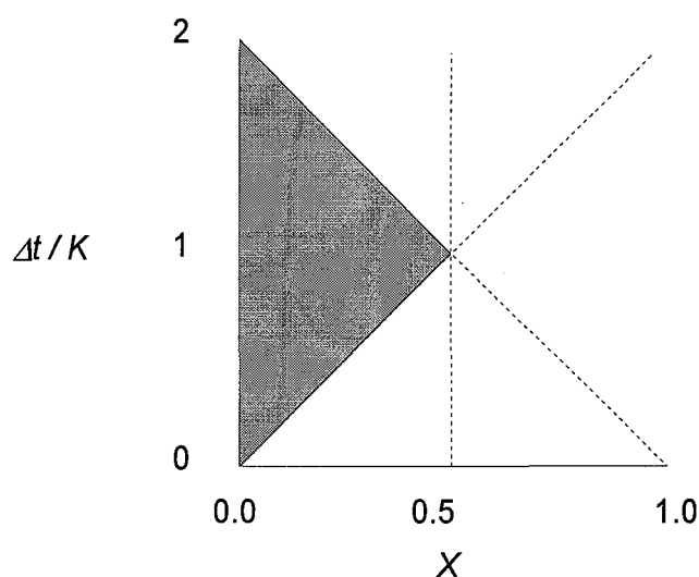
Figure 8-3. Feasible region for Muskingum model parameters
