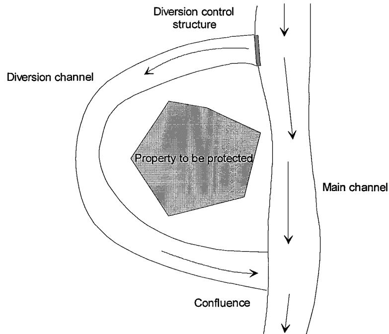
Figure 10-2. Illustration of diversion return flow
