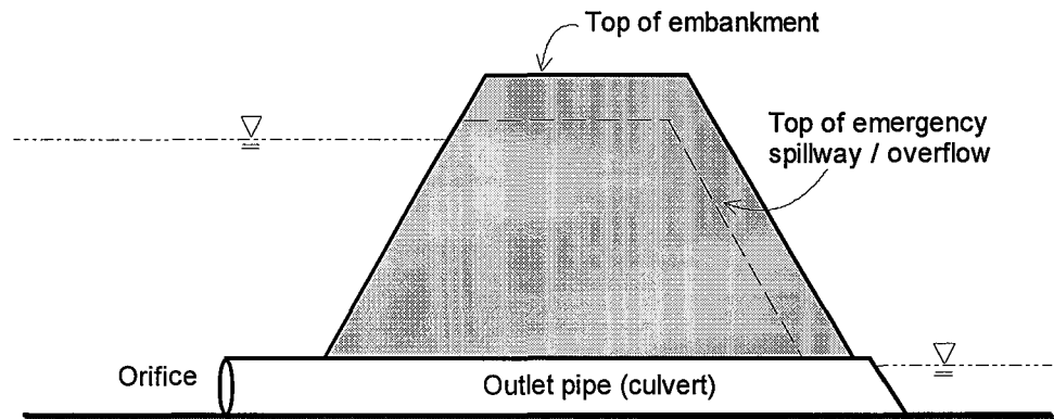
Figure 10-4. Simple detention structure
