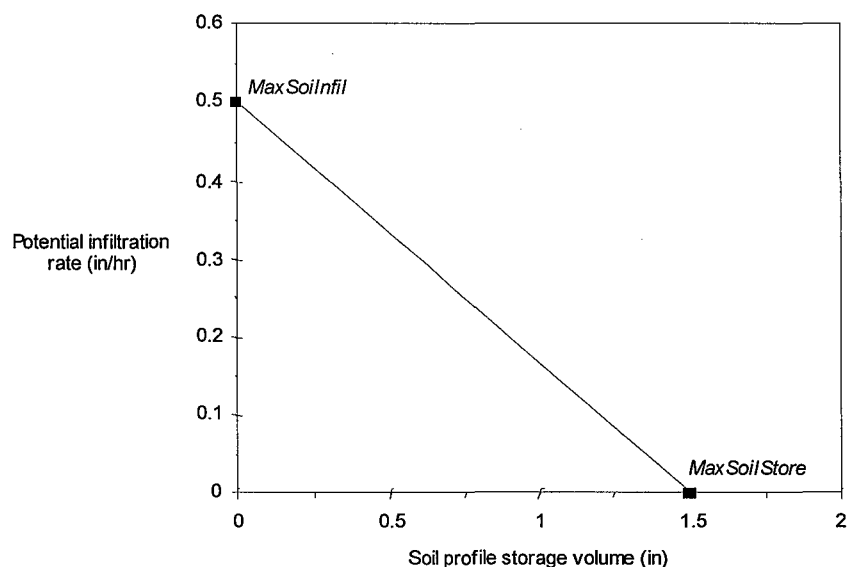
Figure 5-3. Potential infiltration rate versus beginning of time step soil profile storage
