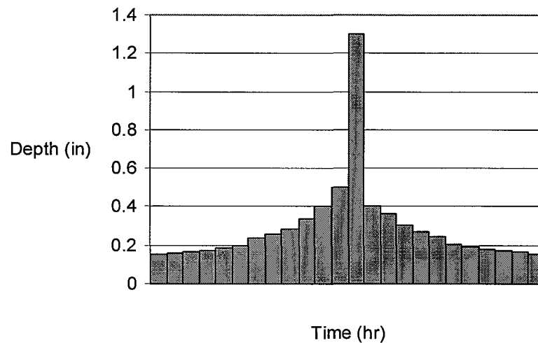
Figure 4-10. Example of distribution of frequency-based hypothetical storm
