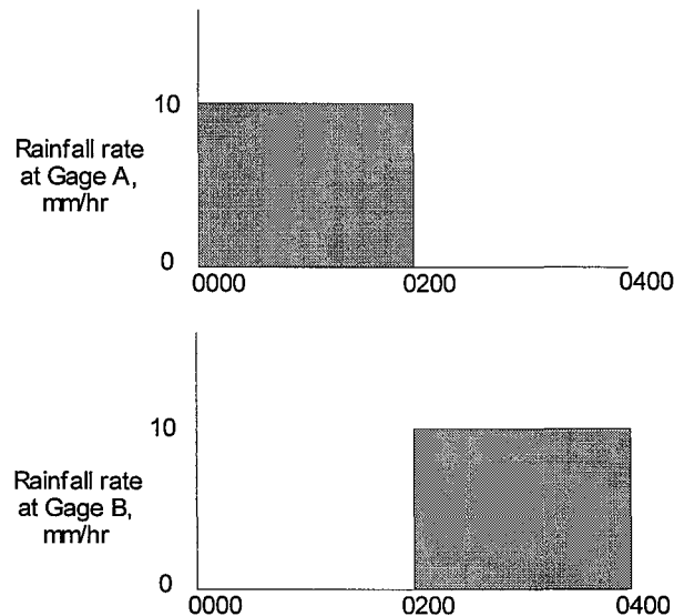
Figure 4-4. Illustration of hazard of averaging rainfall temporal distributions
