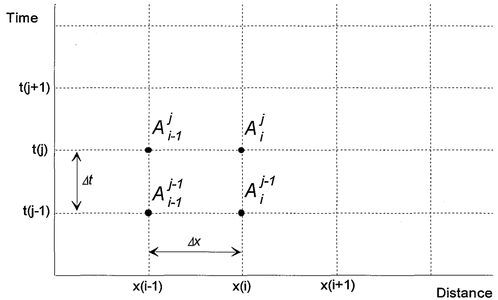
Figure 6-5. Finite difference method space-time grid
