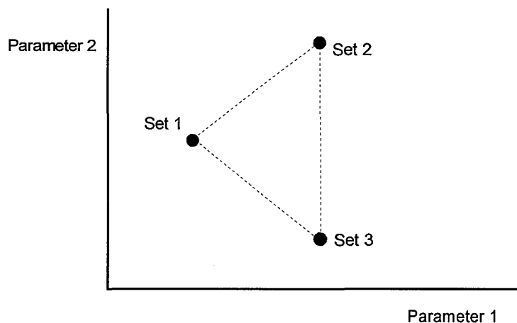
Figure 9-5. Initial simplex for a 2-parameter model
