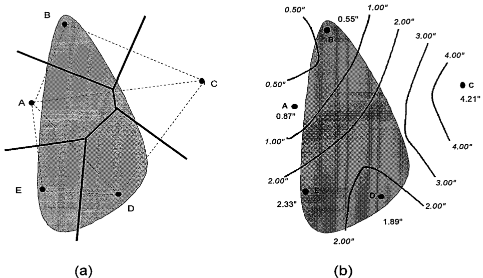
Figure 4-3. Illustration of MAP depth computation schemes
