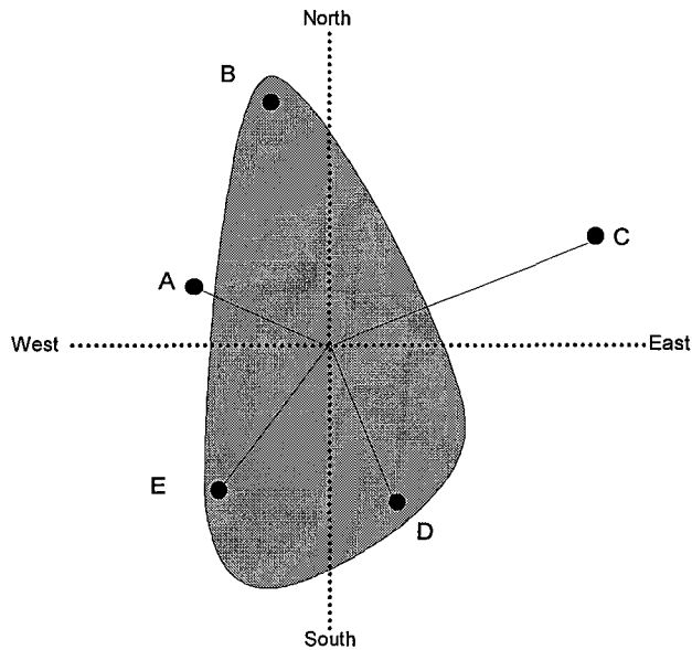
Figure 4-5. Illustration of inverse-distance-squared scheme
