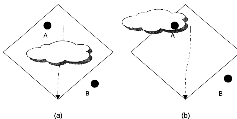
Figure 4-7. Lack of coverage can complicate MAP estimation
