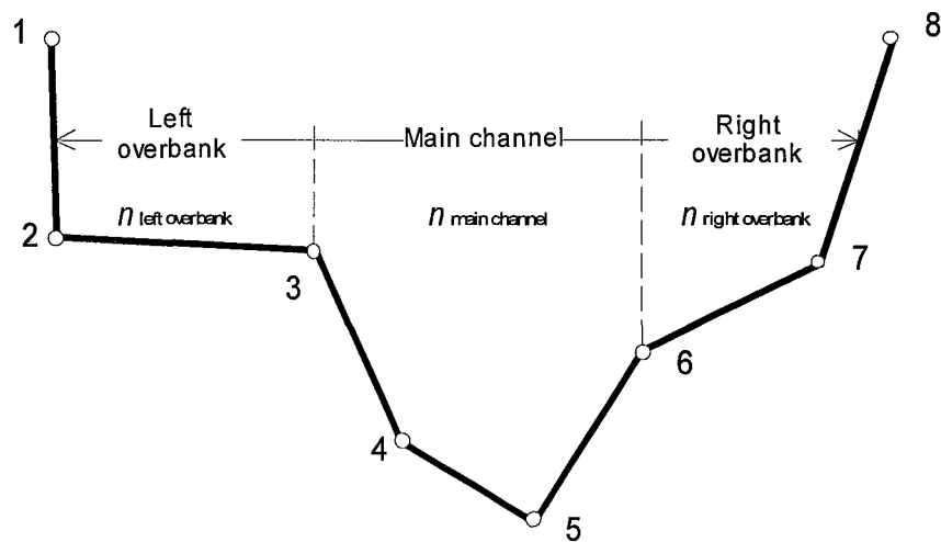
Figure 8-5. Format for describing channel geometry with 8 points
