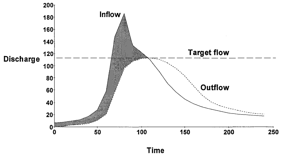
Figure 10-3. Illustration of impact of detention
