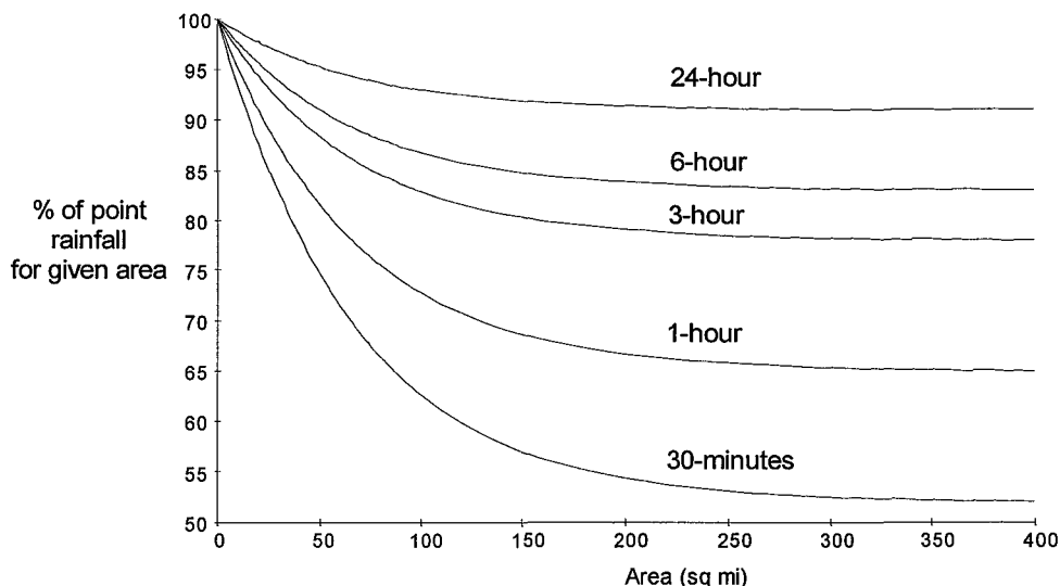
Figure 4-9. Point depth reduction factors
