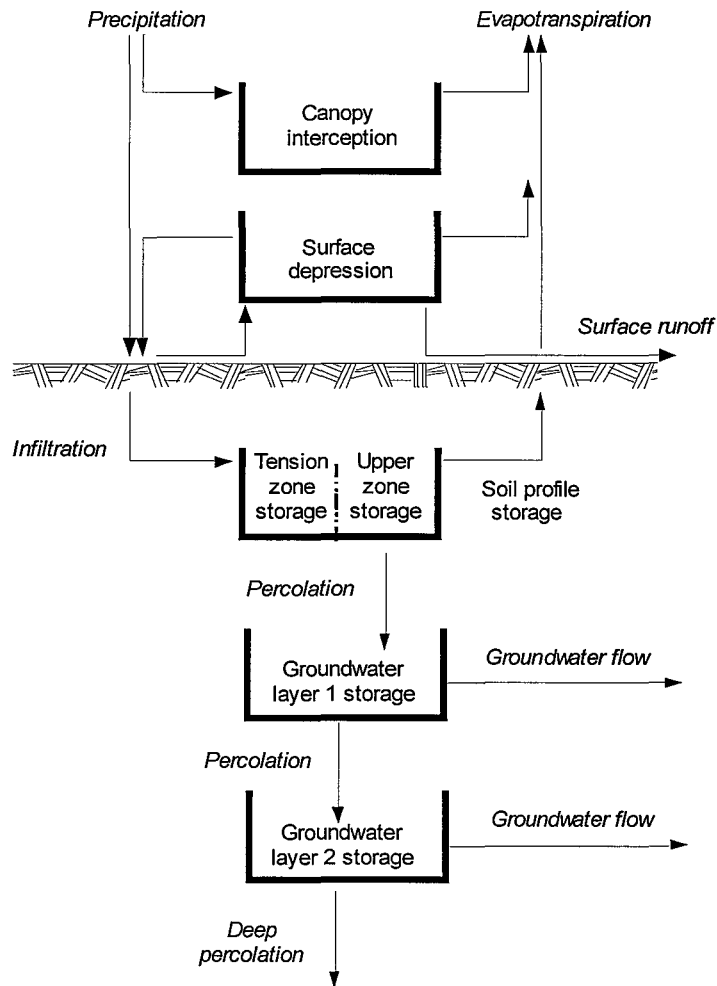
Figure 5-1. Conceptual schematic of the continuous soil moisture accounting algorithm (Bennett, 1998)
