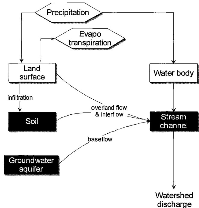
Figure 3-2. Typical HEC-HMS representation of watershed runoff
