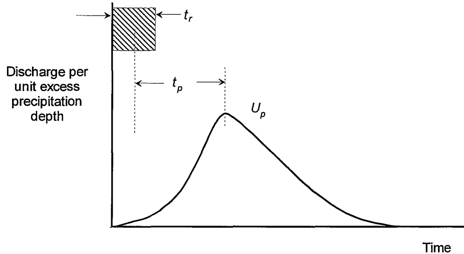
Figure 6-1. Snyder's unit hydrograph
