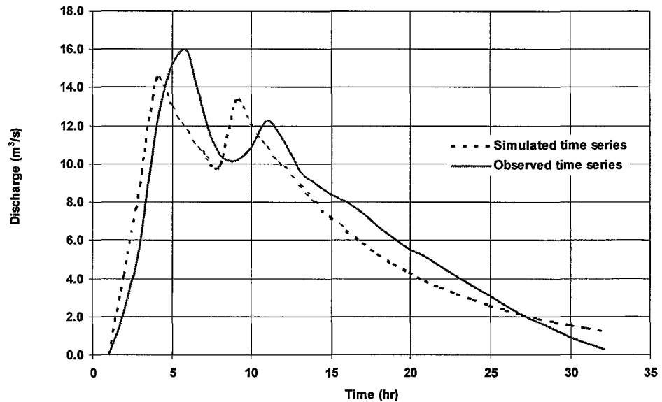
Figure 9-2. How well does the computed hydrograph "fit"?
