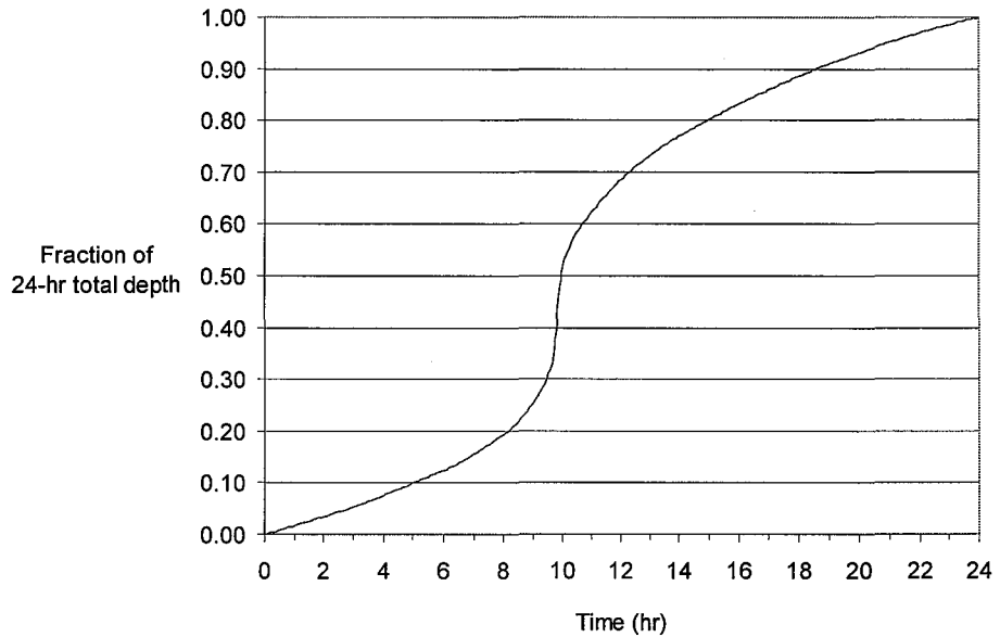
Figure 4-11. SCS hypothetical storm distribution
