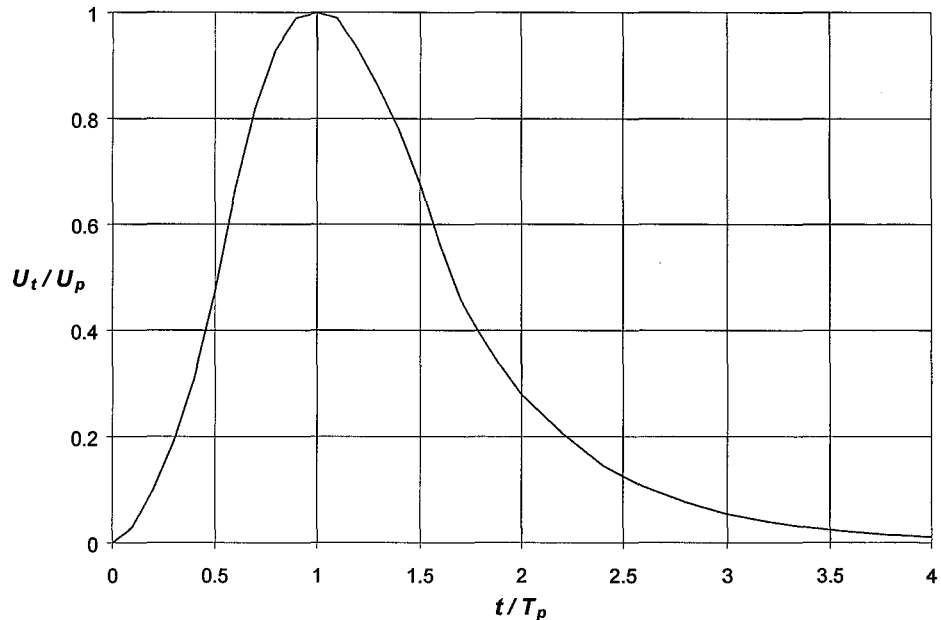
Figure 6-2. SCS unit hydrograph
