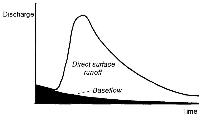
Figure 7-1. Initial baseflow recession
