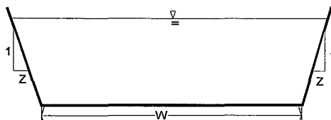
Trapezoidal section
