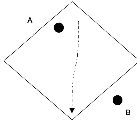
Figure 4-6. MAP can be computed as a weighted-average of depths at gages A and B
