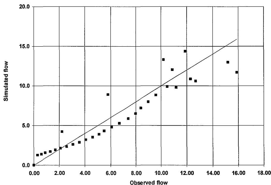
Figure 9-3. Scatter plot
