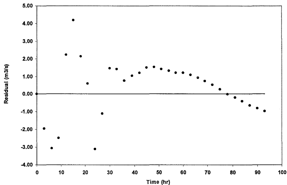
Figure 9-4. Residual plot
